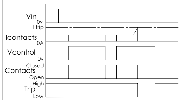
Timing Diagram
